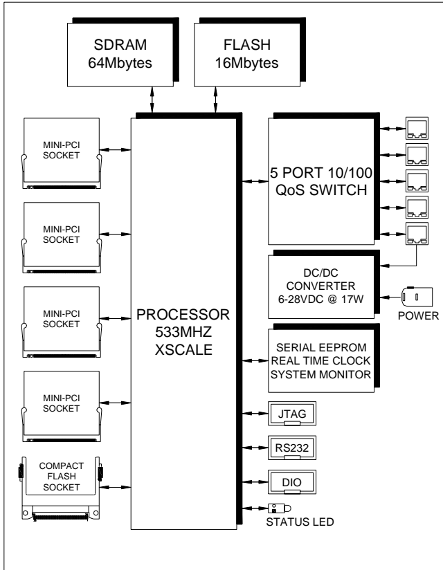
Avila GW2345 Functional Diagram
